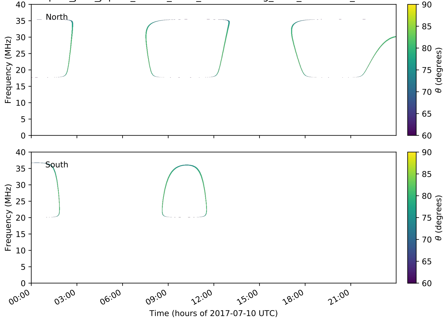
expres_juno_jupiter_17d-0r_isaac_lossc-wid1deg_5kev_20170710_v01.cdf
