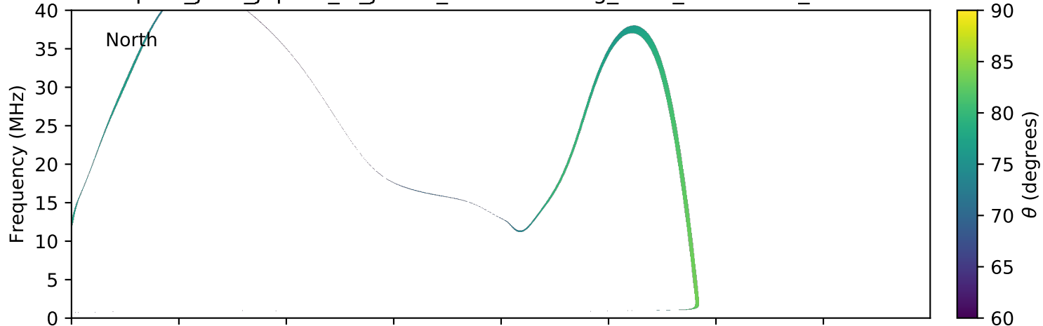
expres_juno_jupiter_io_jrm09_lossc-wid1deg_3kev_20170628_v01.cdf
