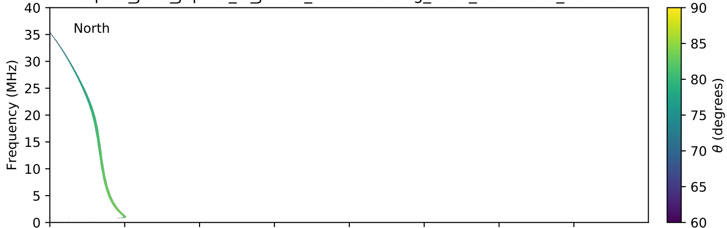
expres_juno_jupiter_io_jrm09_lossc-wid1deg_3kev_20170625_v01.cdf
