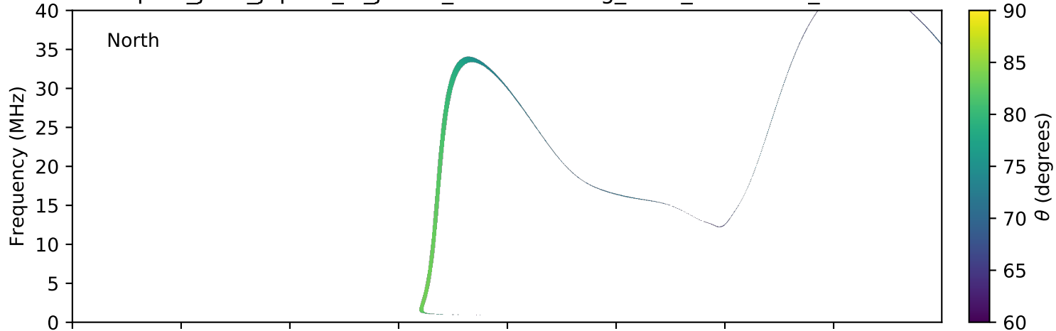
expres_juno_jupiter_io_jrm09_lossc-wid1deg_3kev_20170624_v01.cdf
