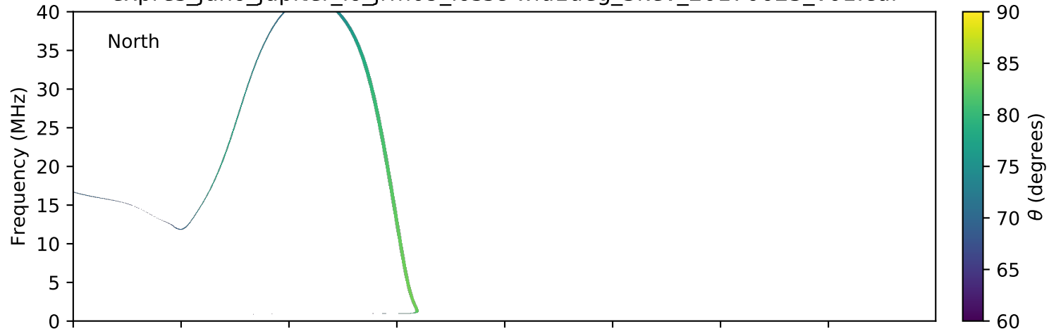
expres_juno_jupiter_io_jrm09_lossc-wid1deg_3kev_20170623_v01.cdf
