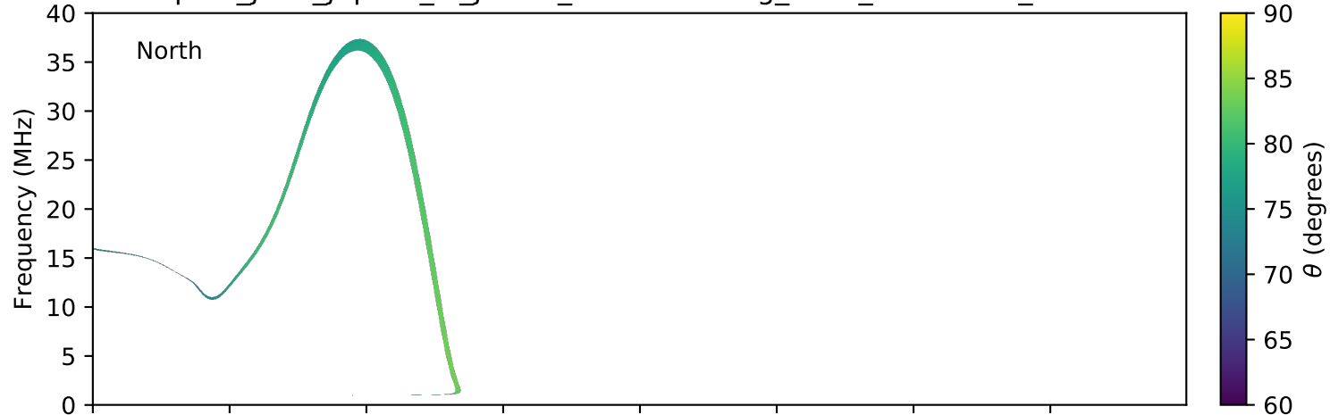
expres_juno_jupiter_io_jrm09_lossc-wid1deg_3kev_20170616_v01.cdf
