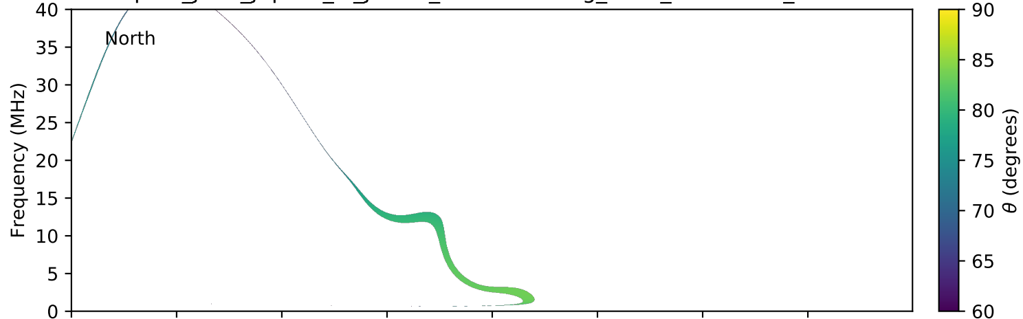
expres_juno_jupiter_io_jrm09_lossc-wid1deg_3kev_20170614_v01.cdf
