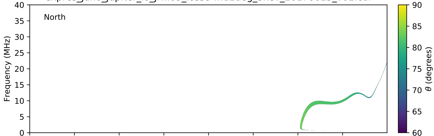
expres_juno_jupiter_io_jrm09_lossc-wid1deg_3kev_20170613_v01.cdf
