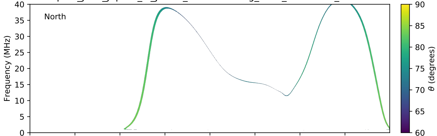
expres_juno_jupiter_io_jrm09_lossc-wid1deg_3kev_20170610_v01.cdf
