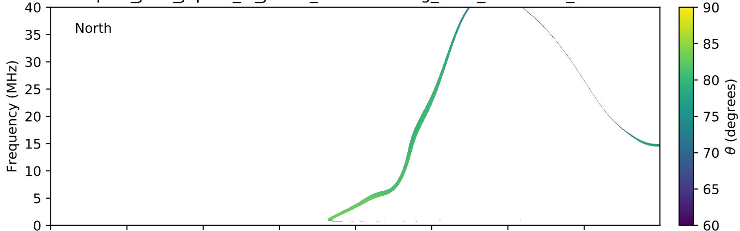
expres_juno_jupiter_io_jrm09_lossc-wid1deg_3kev_20170608_v01.cdf
