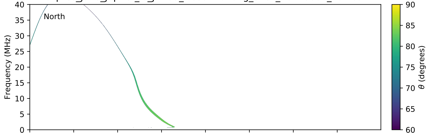
expres_juno_jupiter_io_jrm09_lossc-wid1deg_3kev_20170607_v01.cdf
