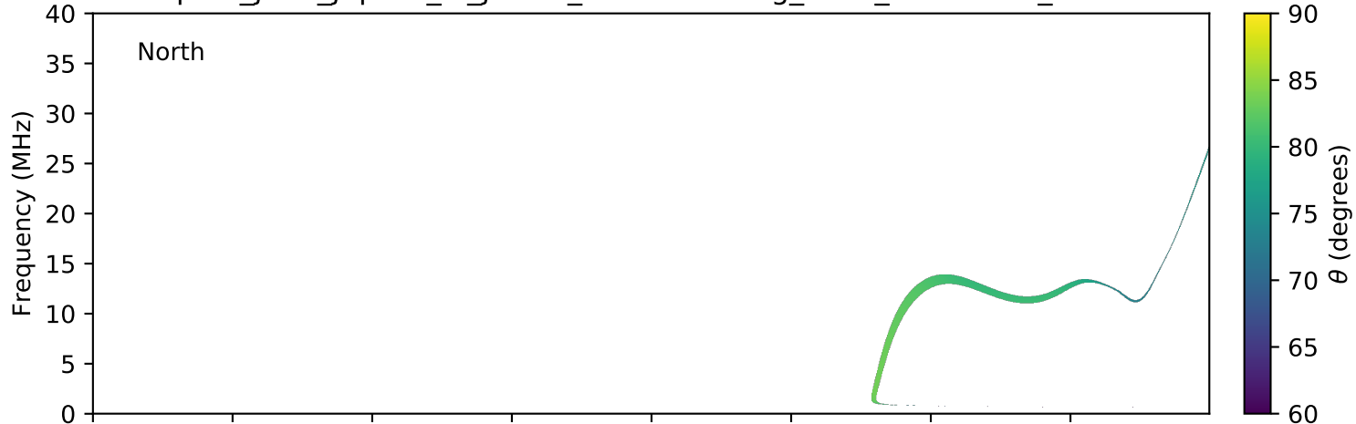
expres_juno_jupiter_io_jrm09_lossc-wid1deg_3kev_20170606_v01.cdf
