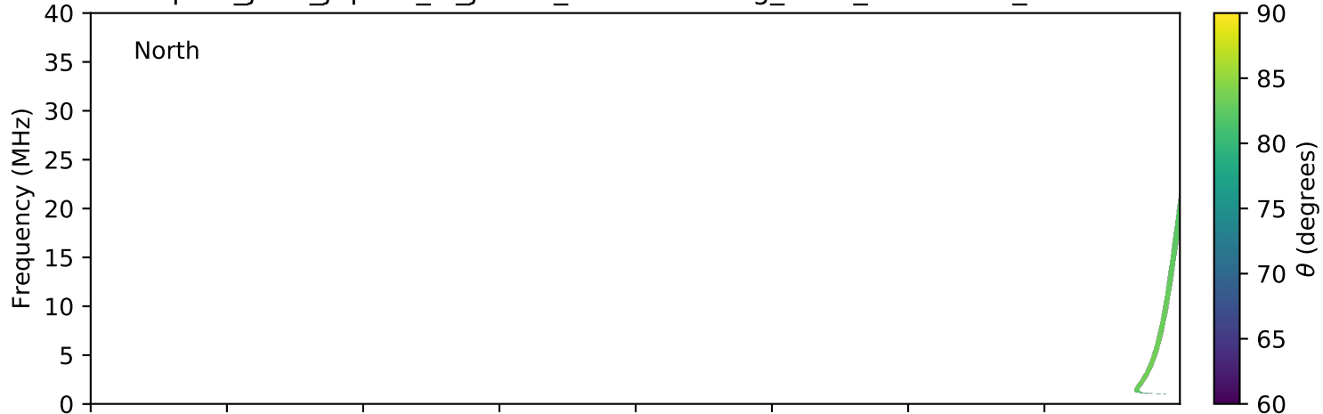
expres_juno_jupiter_io_jrm09_lossc-wid1deg_3kev_20170604_v01.cdf
