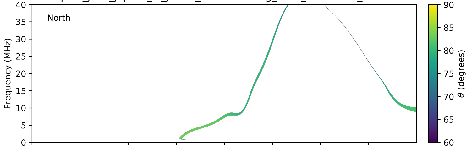
expres_juno_jupiter_io_jrm09_lossc-wid1deg_3kev_20170601_v01.cdf
