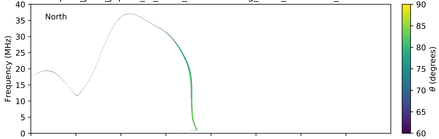
expres_juno_jupiter_io_isaac_lossc-wid1deg_3kev_20170630_v01.cdf
