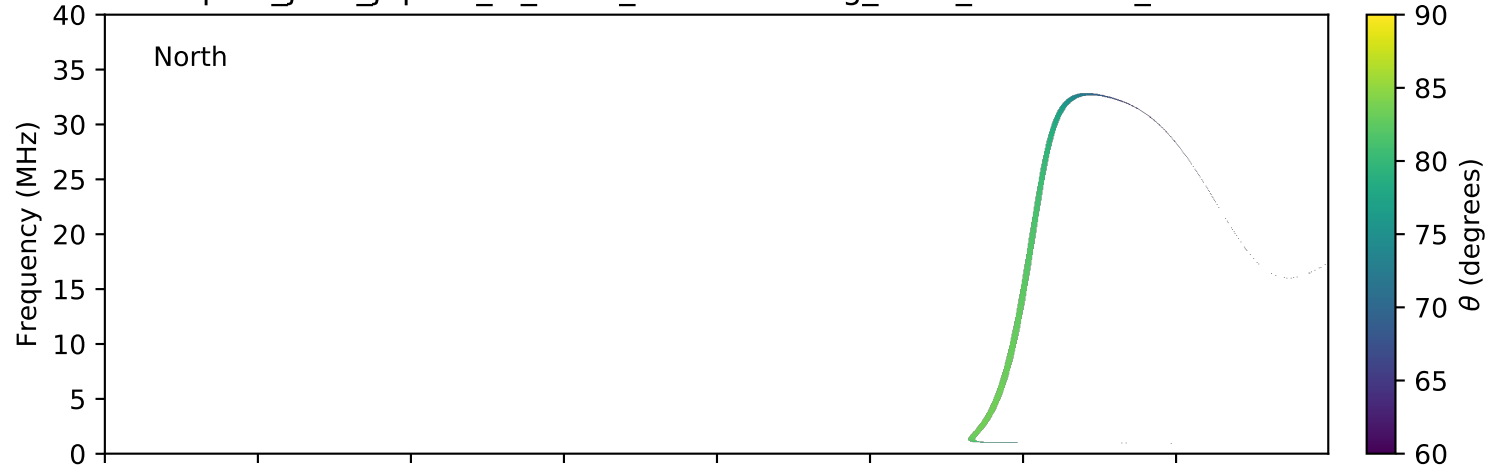
expres_juno_jupiter_io_isaac_lossc-wid1deg_3kev_20170629_v01.cdf
