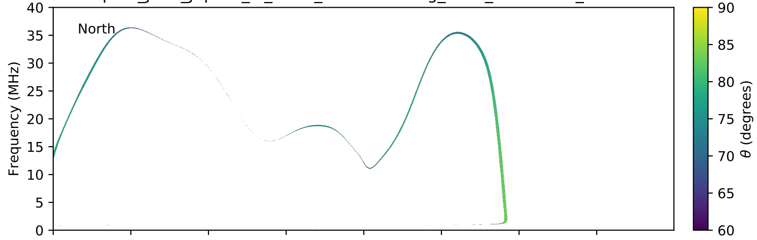
expres_juno_jupiter_io_isaac_lossc-wid1deg_3kev_20170628_v01.cdf
