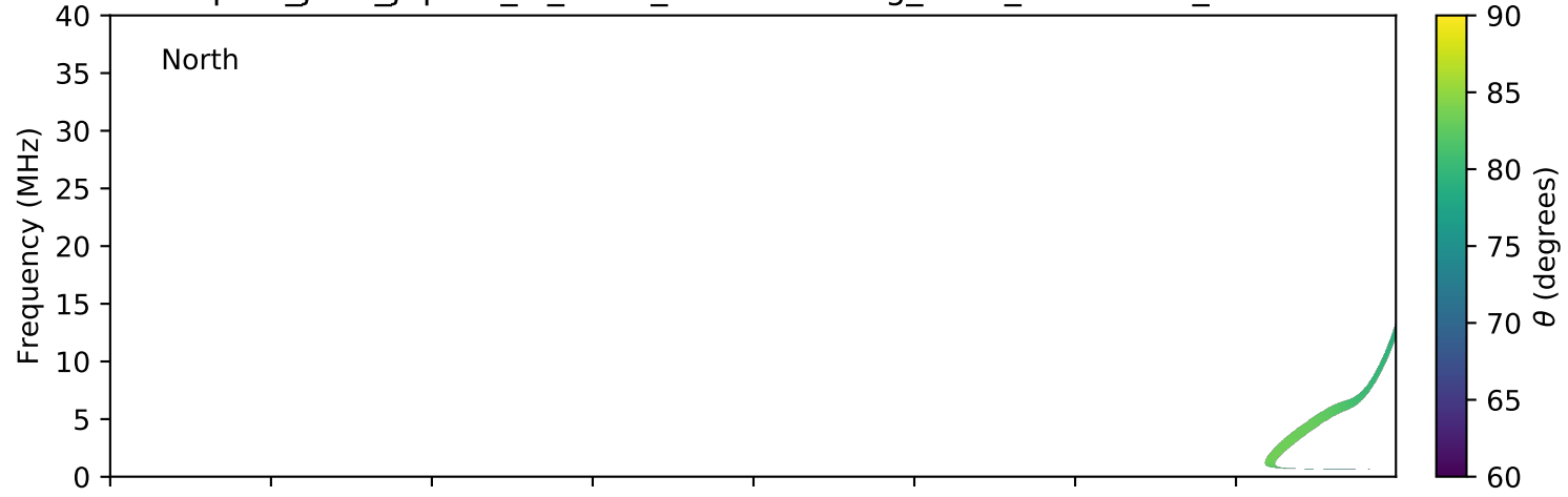
expres_juno_jupiter_io_isaac_lossc-wid1deg_3kev_20170627_v01.cdf
