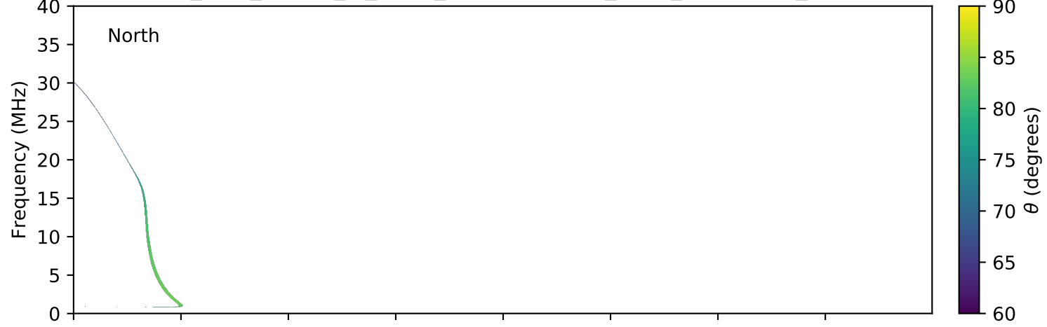
expres_juno_jupiter_io_isaac_lossc-wid1deg_3kev_20170625_v01.cdf
