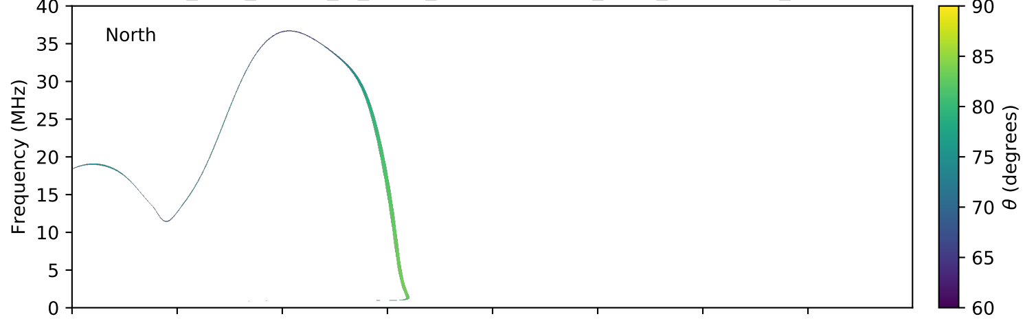
expres_juno_jupiter_io_isaac_lossc-wid1deg_3kev_20170623_v01.cdf
