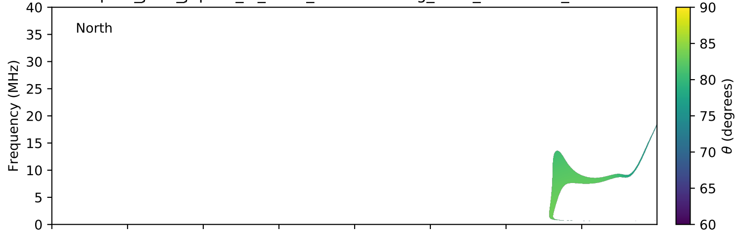
expres_juno_jupiter_io_isaac_lossc-wid1deg_3kev_20170620_v01.cdf
