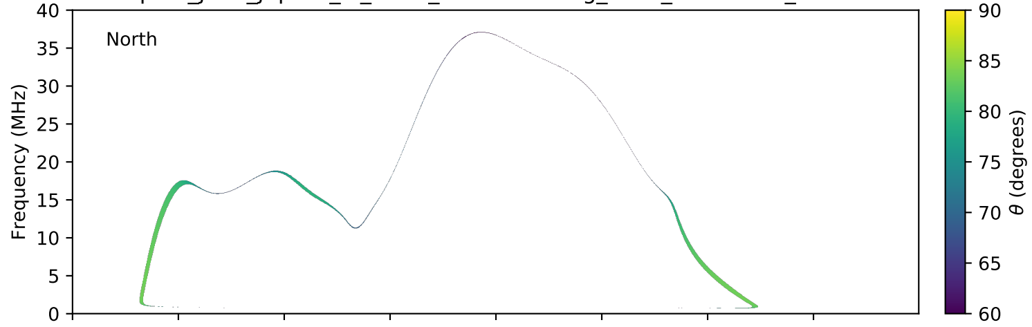
expres_juno_jupiter_io_isaac_lossc-wid1deg_3kev_20170619_v01.cdf
