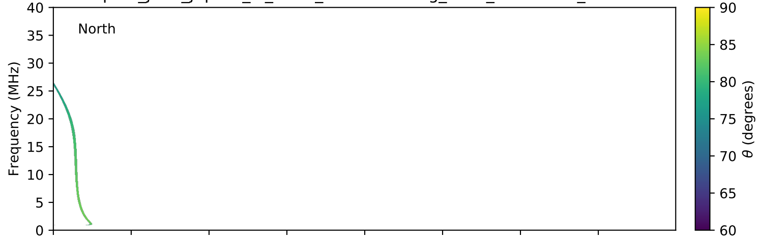
expres_juno_jupiter_io_isaac_lossc-wid1deg_3kev_20170618_v01.cdf
