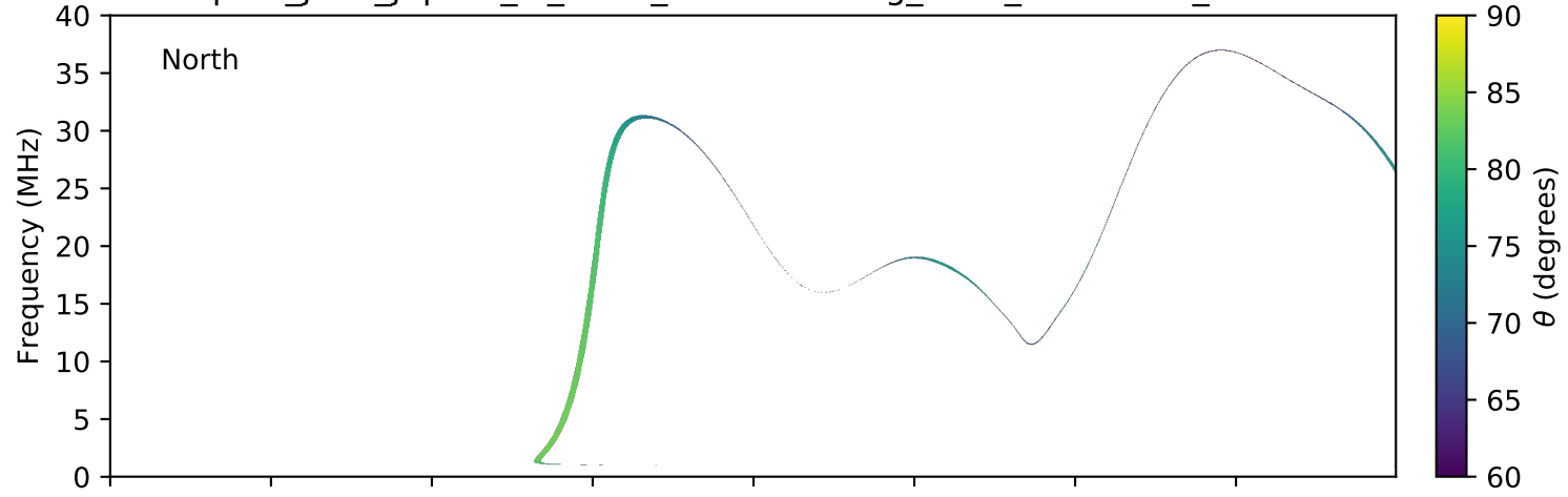
expres_juno_jupiter_io_isaac_lossc-wid1deg_3kev_20170617_v01.cdf
