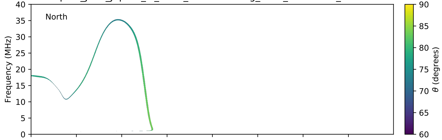
expres_juno_jupiter_io_isaac_lossc-wid1deg_3kev_20170616_v01.cdf
