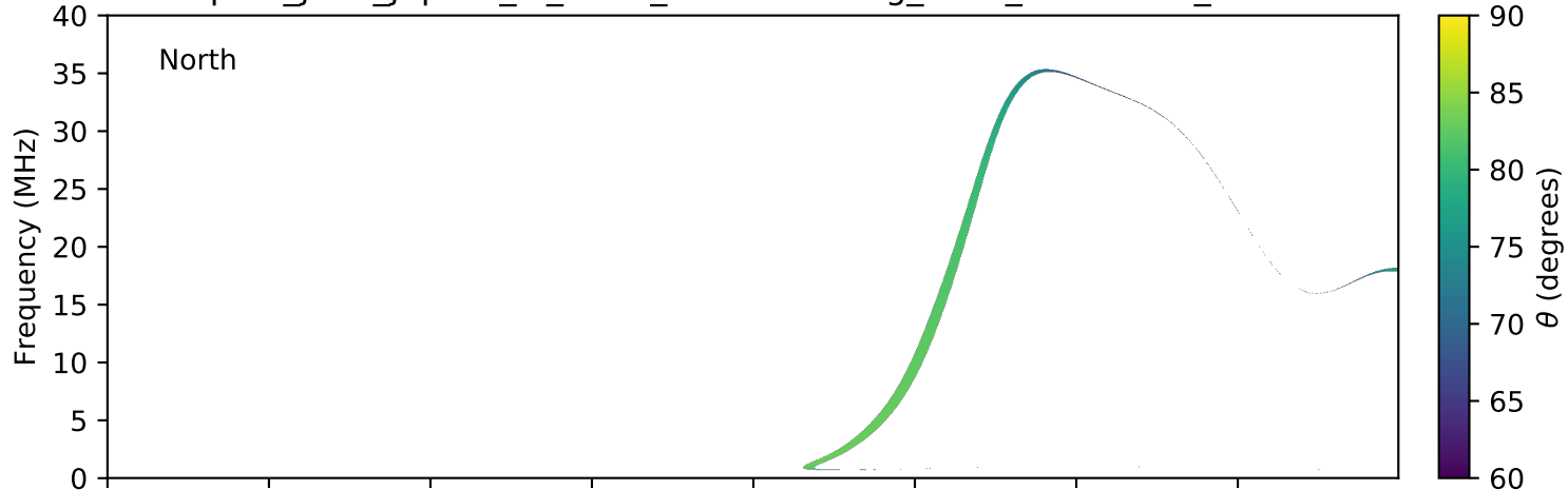
expres_juno_jupiter_io_isaac_lossc-wid1deg_3kev_20170615_v01.cdf
