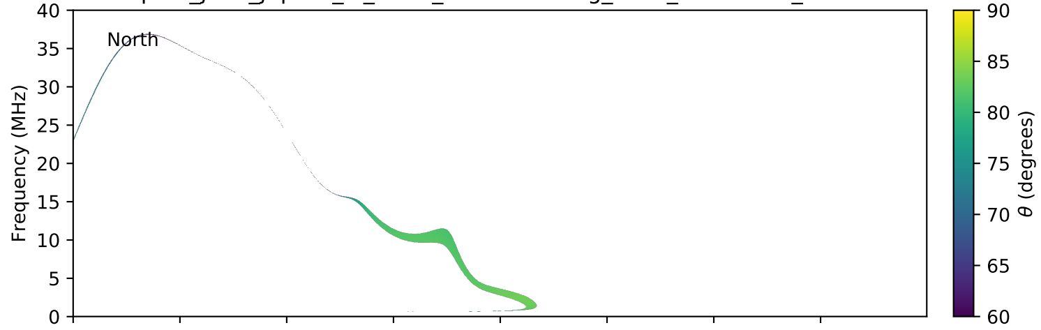
expres_juno_jupiter_io_isaac_lossc-wid1deg_3kev_20170614_v01.cdf
