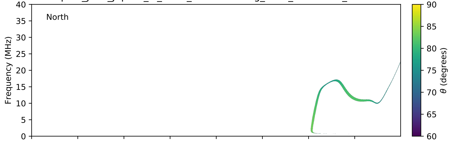
expres_juno_jupiter_io_isaac_lossc-wid1deg_3kev_20170613_v01.cdf
