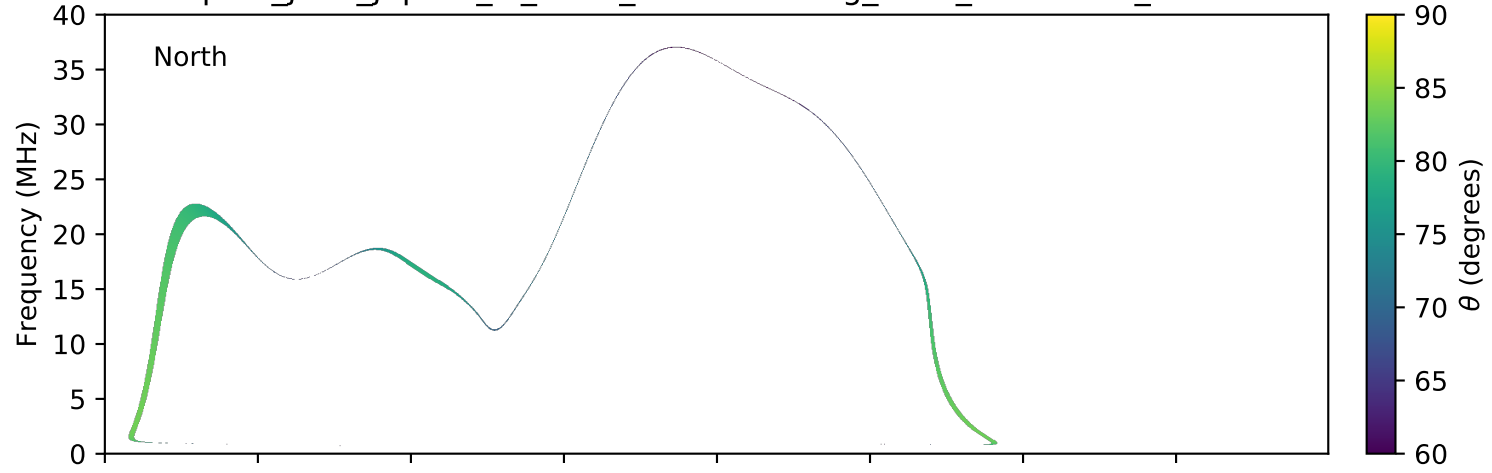
expres_juno_jupiter_io_isaac_lossc-wid1deg_3kev_20170612_v01.cdf
