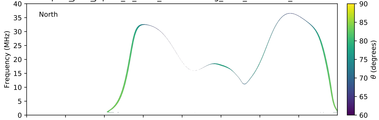
expres_juno_jupiter_io_isaac_lossc-wid1deg_3kev_20170610_v01.cdf
