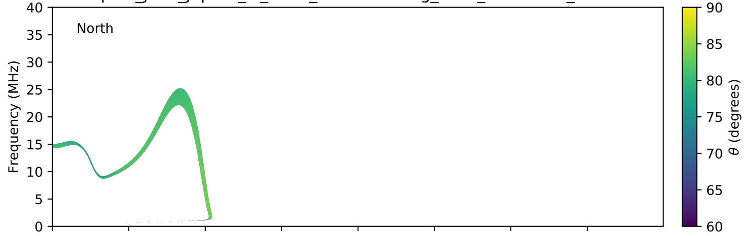
expres_juno_jupiter_io_isaac_lossc-wid1deg_3kev_20170609_v01.cdf
