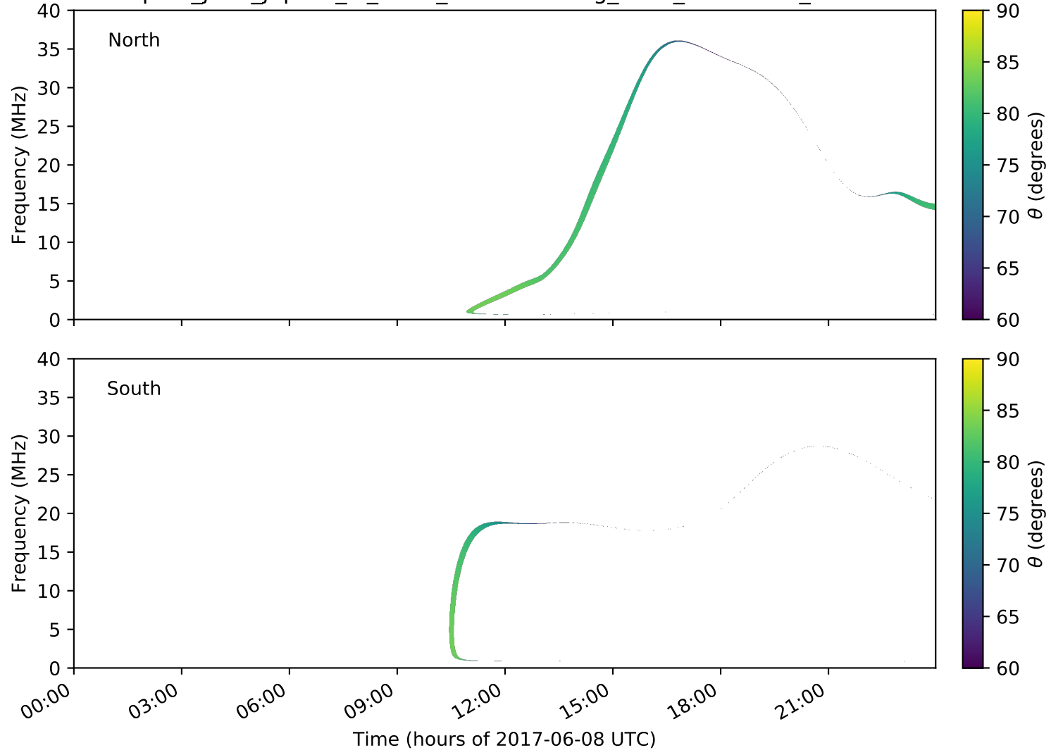
expres_juno_jupiter_io_isaac_lossc-wid1deg_3kev_20170608_v01.cdf
