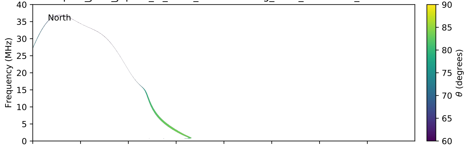
expres_juno_jupiter_io_isaac_lossc-wid1deg_3kev_20170607_v01.cdf
