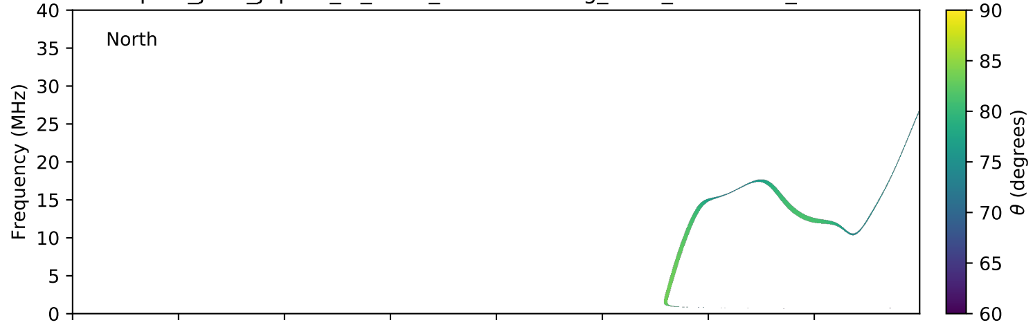
expres_juno_jupiter_io_isaac_lossc-wid1deg_3kev_20170606_v01.cdf
