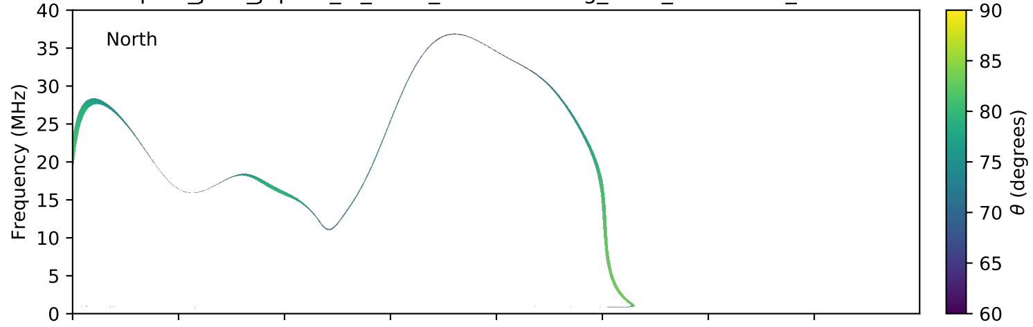
expres_juno_jupiter_io_isaac_lossc-wid1deg_3kev_20170605_v01.cdf
