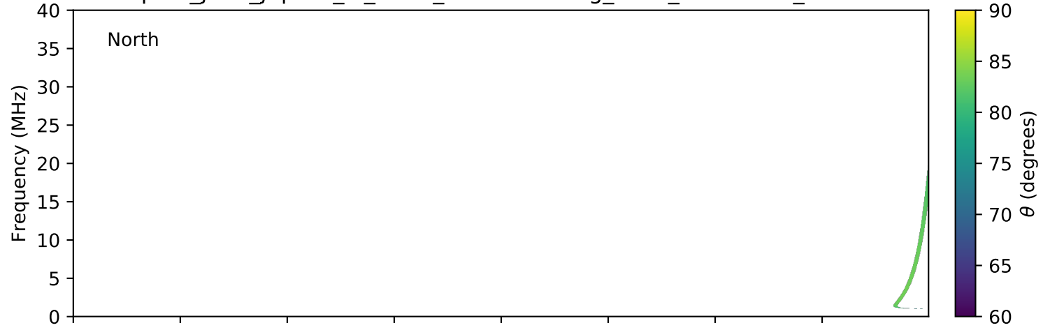
expres_juno_jupiter_io_isaac_lossc-wid1deg_3kev_20170604_v01.cdf
