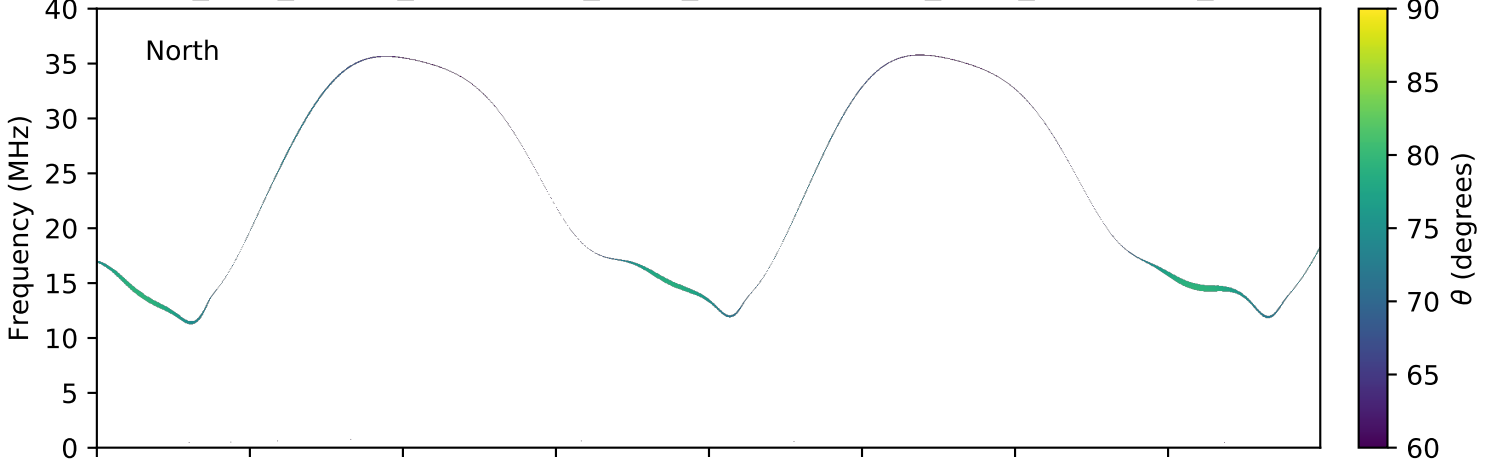
expres_juno_jupiter_ganymede_isaac_lossc-wid1deg_3kev_20170630_v01.cdf
