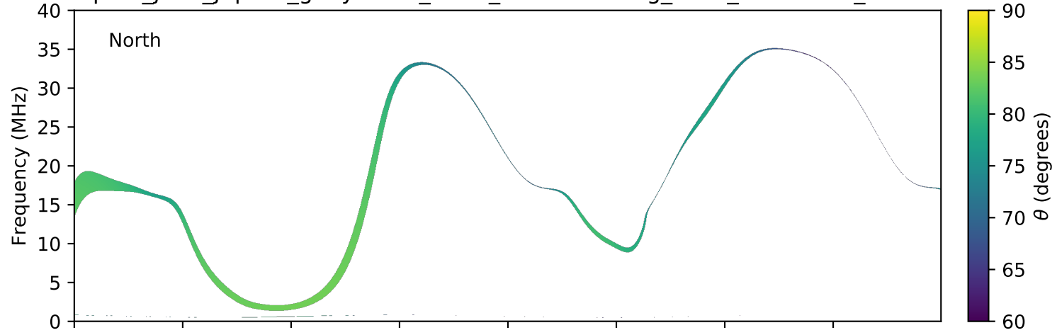
expres_juno_jupiter_ganymede_isaac_lossc-wid1deg_3kev_20170629_v01.cdf
