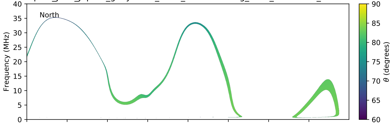
expres_juno_jupiter_ganymede_isaac_lossc-wid1deg_3kev_20170624_v01.cdf
