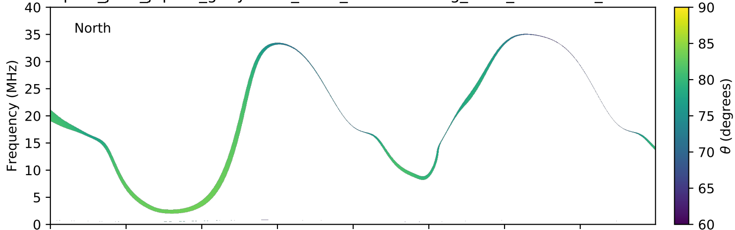
expres_juno_jupiter_ganymede_isaac_lossc-wid1deg_3kev_20170622_v01.cdf
