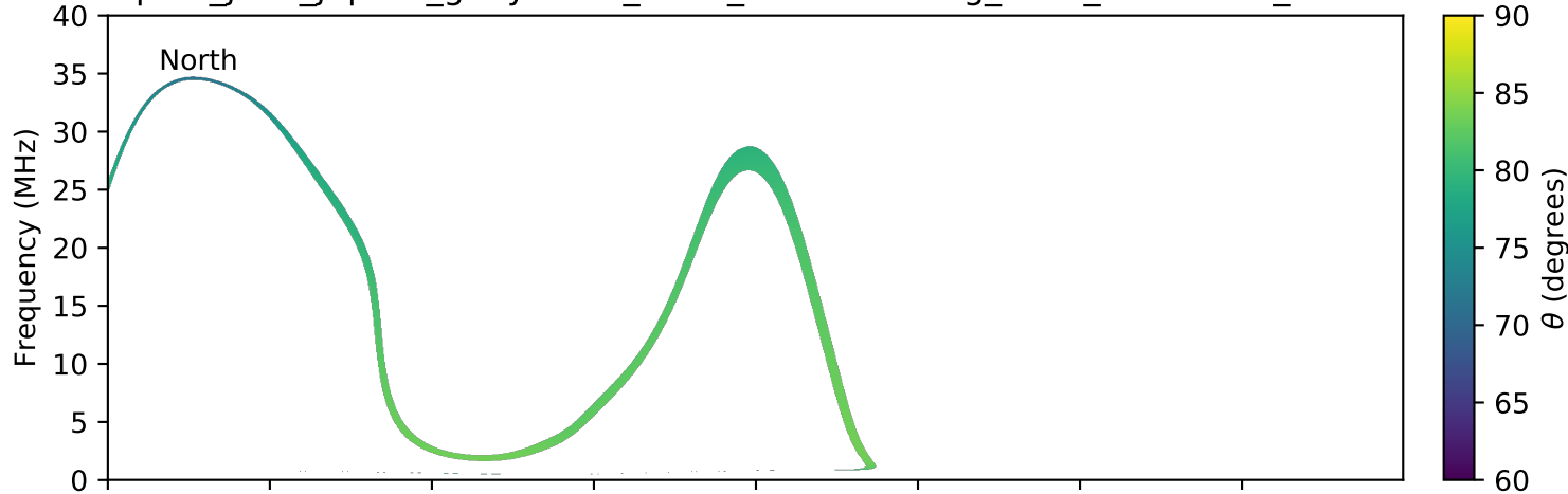
expres_juno_jupiter_ganymede_isaac_lossc-wid1deg_3kev_20170617_v01.cdf
