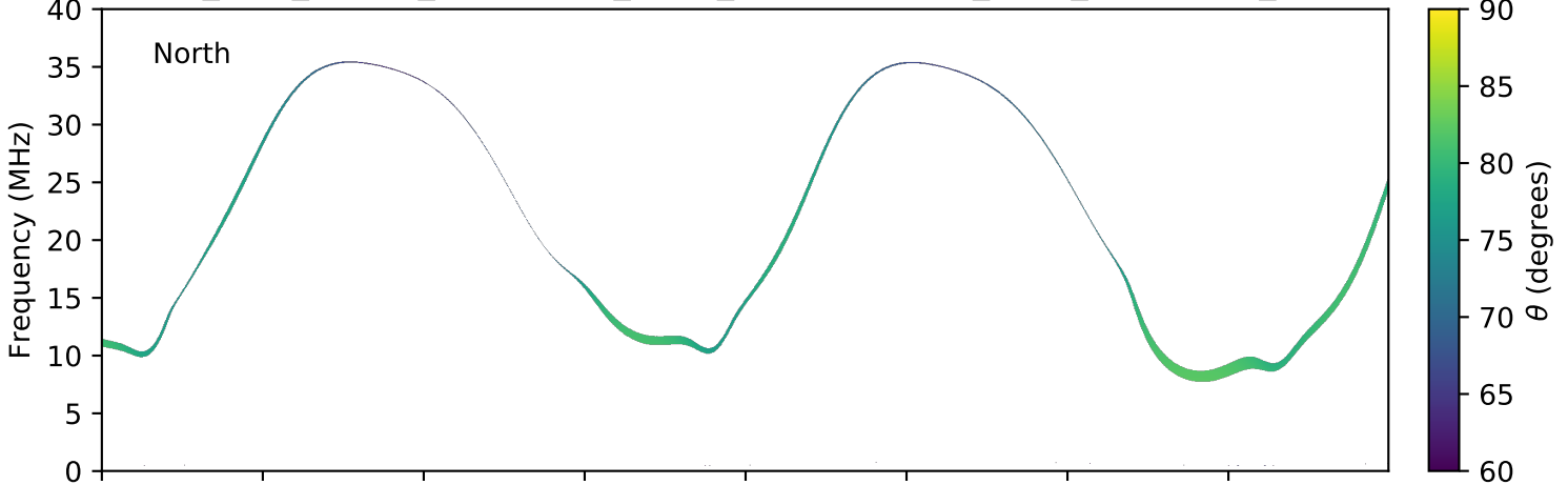
expres_juno_jupiter_ganymede_isaac_lossc-wid1deg_3kev_20170616_v01.cdf
