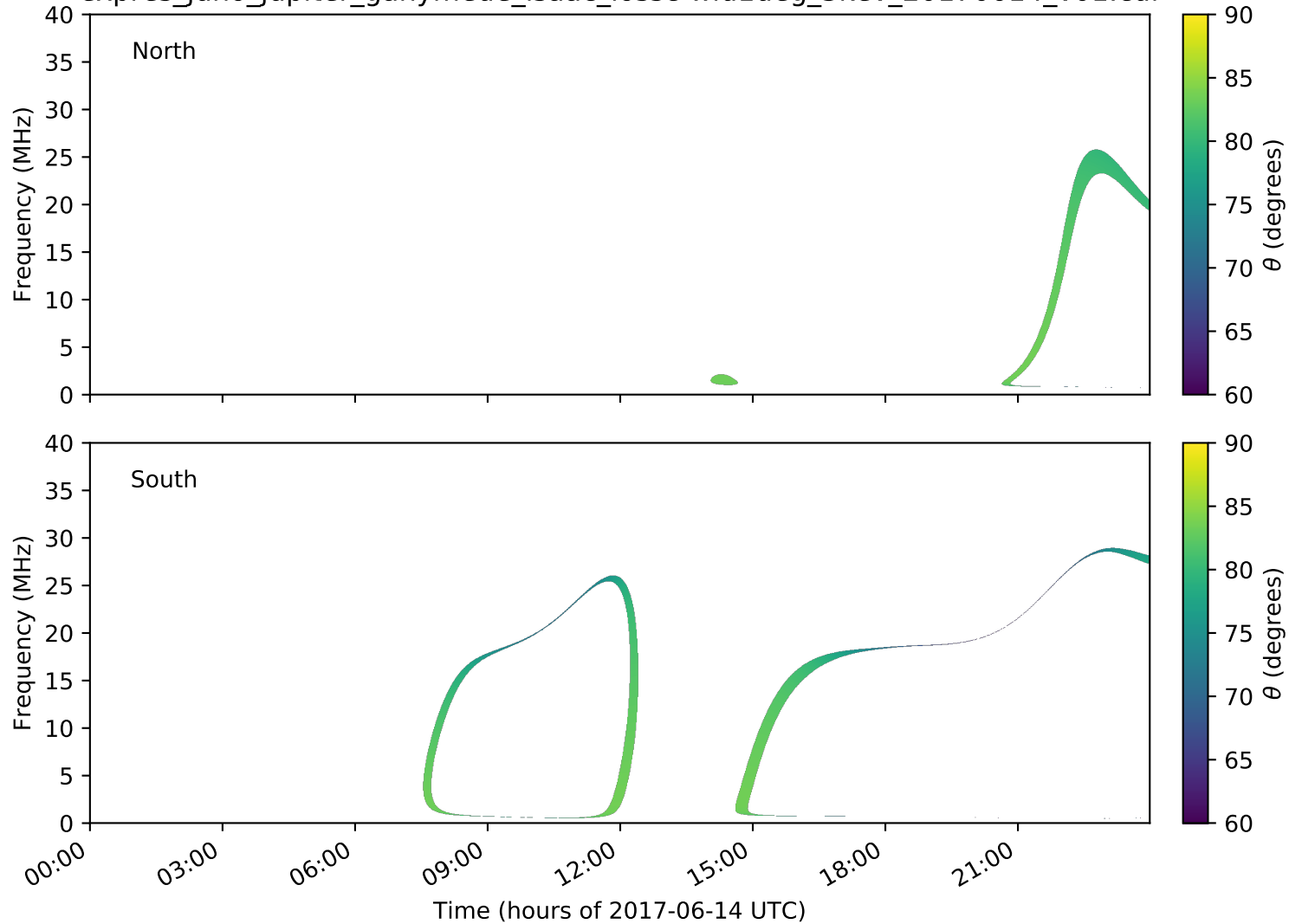
expres_juno_jupiter_ganymede_isaac_lossc-wid1deg_3kev_20170614_v01.cdf
