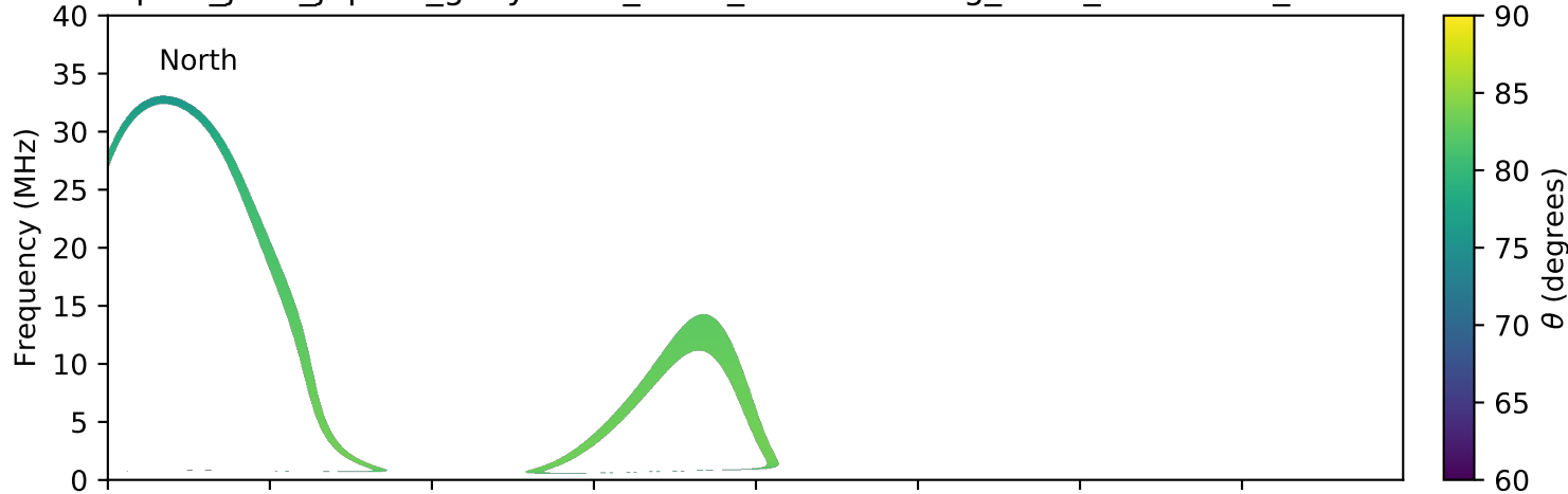
expres_juno_jupiter_ganymede_isaac_lossc-wid1deg_3kev_20170610_v01.cdf
