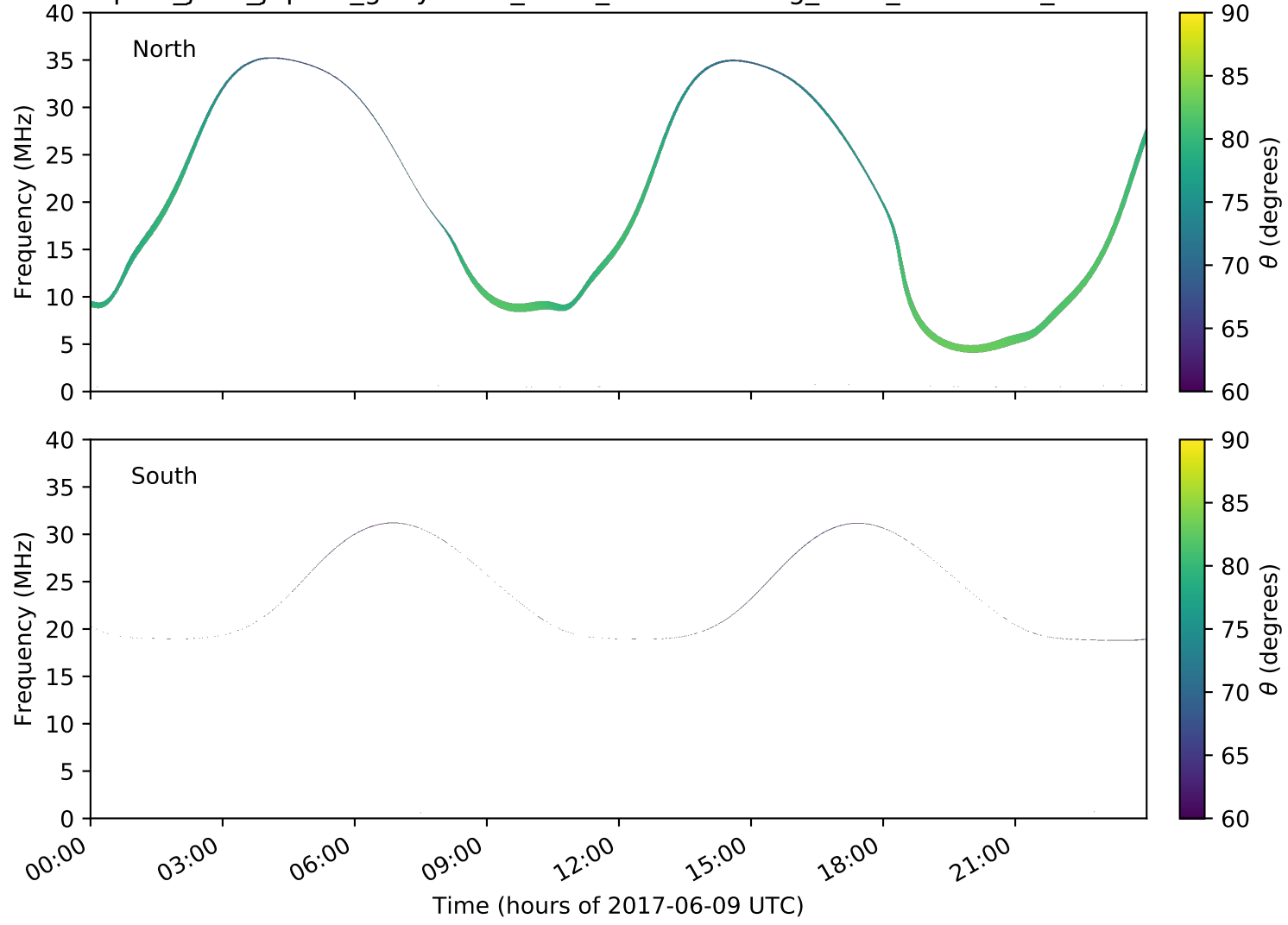
expres_juno_jupiter_ganymede_isaac_lossc-wid1deg_3kev_20170609_v01.cdf
