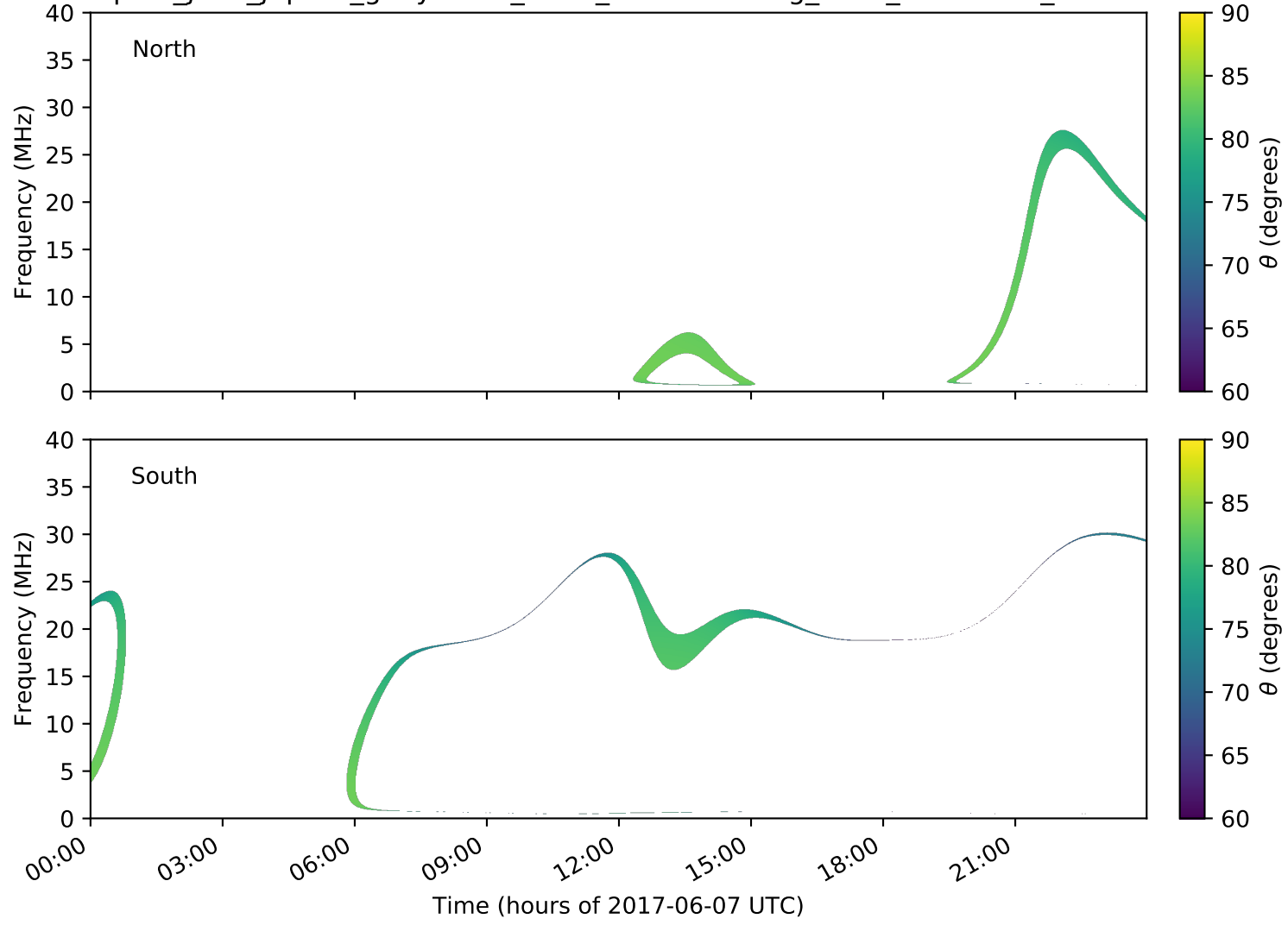
expres_juno_jupiter_ganymede_isaac_lossc-wid1deg_3kev_20170607_v01.cdf
