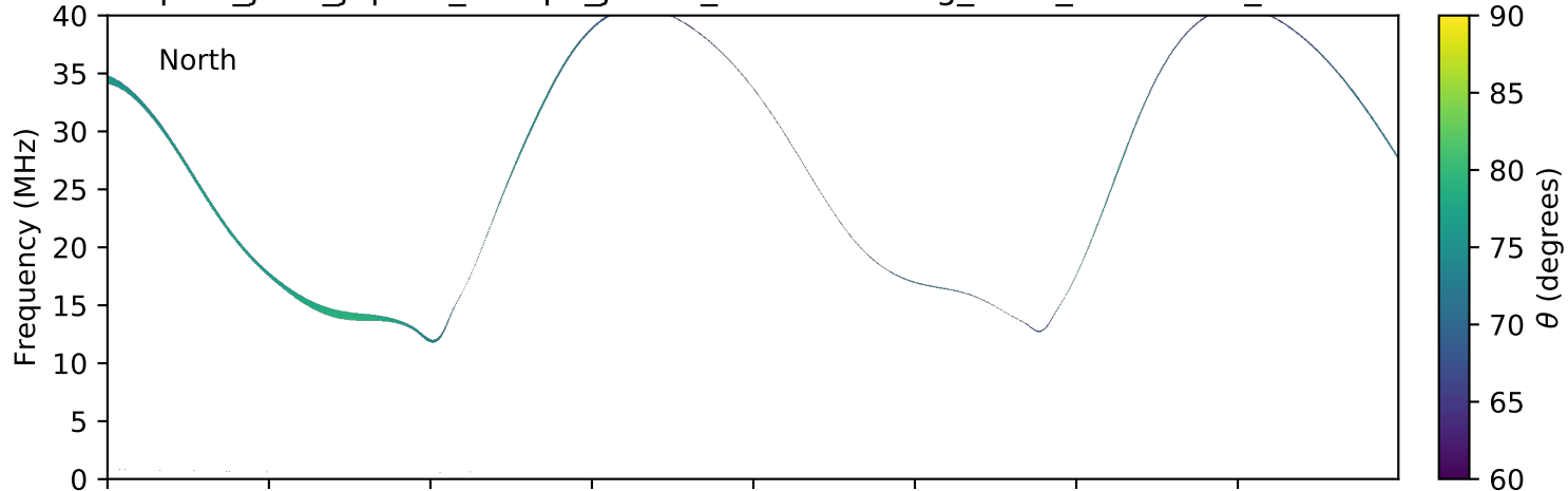
expres_juno_jupiter_europa_jrm09_lossc-wid1deg_3kev_20170629_v01.cdf
