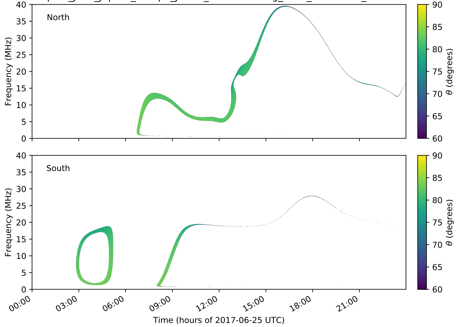
expres_juno_jupiter_europa_jrm09_lossc-wid1deg_3kev_20170625_v01.cdf
