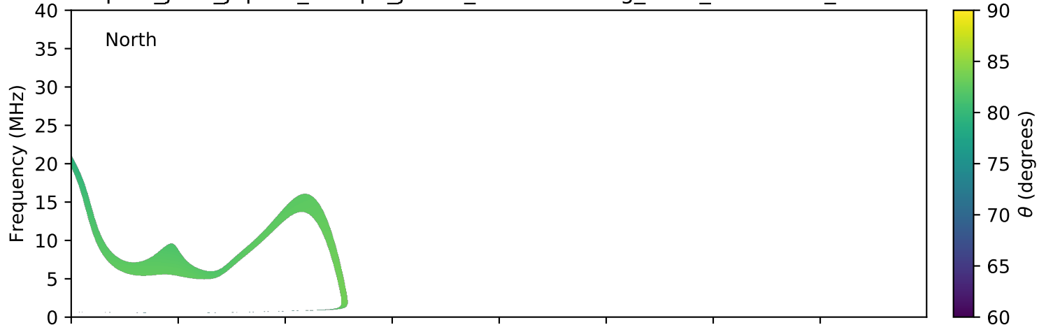
expres_juno_jupiter_europa_jrm09_lossc-wid1deg_3kev_20170623_v01.cdf
