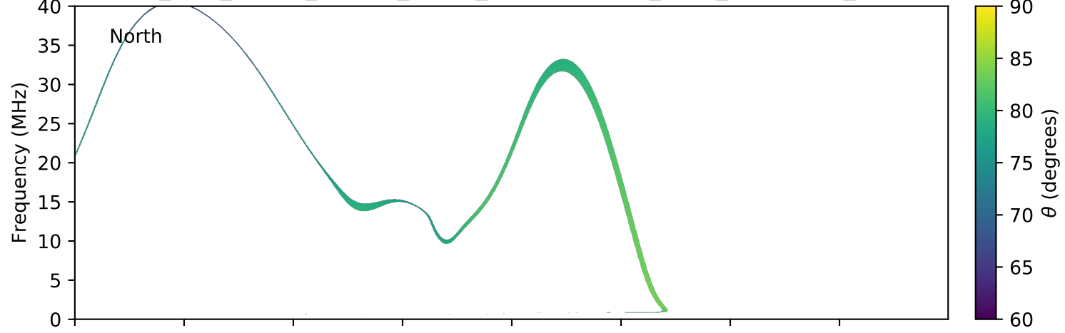
expres_juno_jupiter_europa_jrm09_lossc-wid1deg_3kev_20170619_v01.cdf
